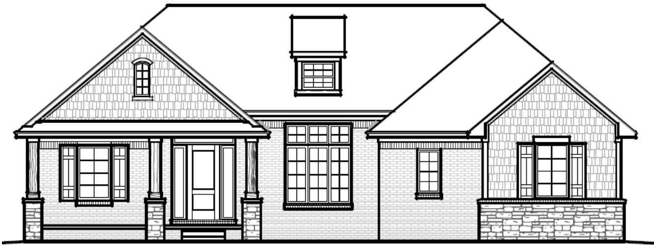
FRONT ELEVATION "B"
